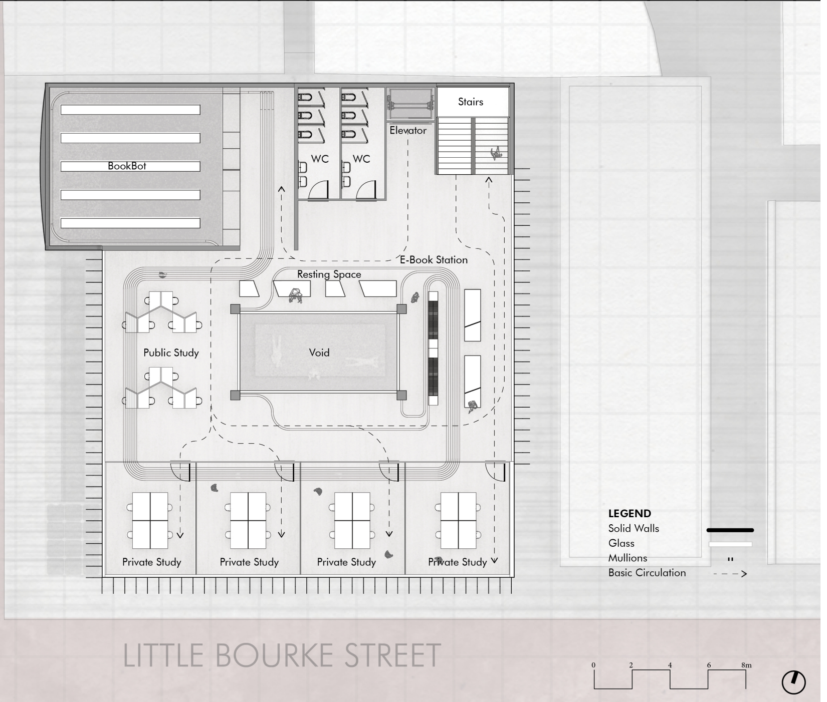
Second Floor Plan - 1-200
